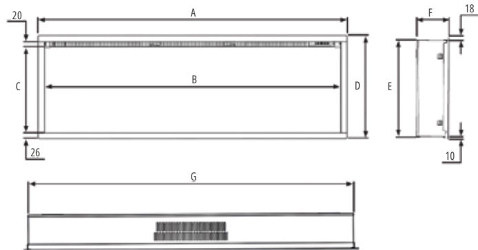
Atmos Slim Dimensions
