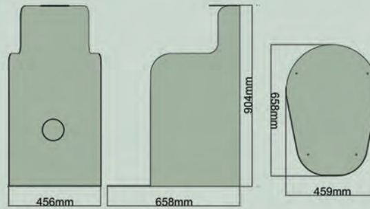
ApplePie Tall Enclosure
