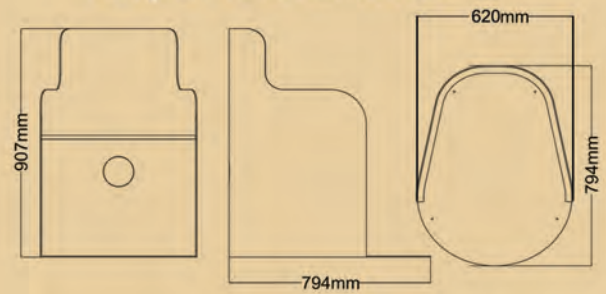
PumpkinPie Tall Enclosure
