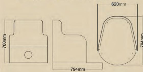
PumpkinPie Low Enclosure
